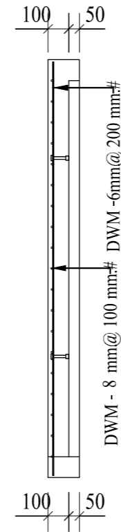
A - A (1:25)
