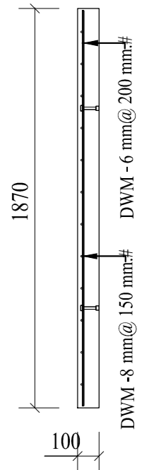
A - A (1:25)
