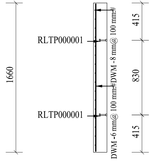
A - A (1:25)
