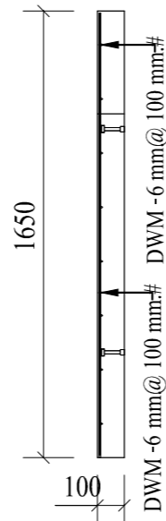
A - A (1:25)
