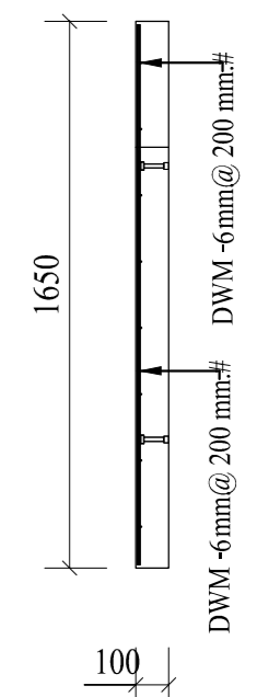
A - A (1:25)
