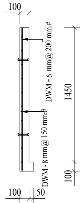
A - A (1:25)
