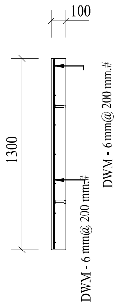
A - A (1:25)
