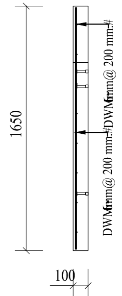
A - A (1:25)
