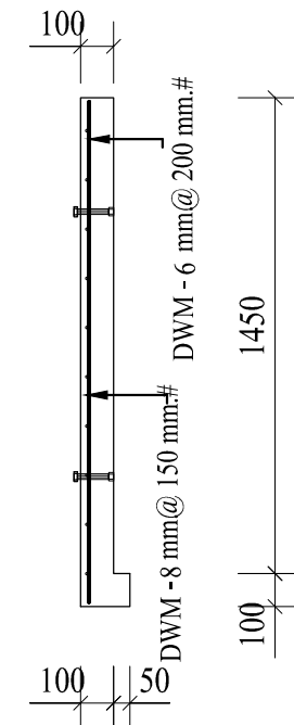
A - A (1:25)
