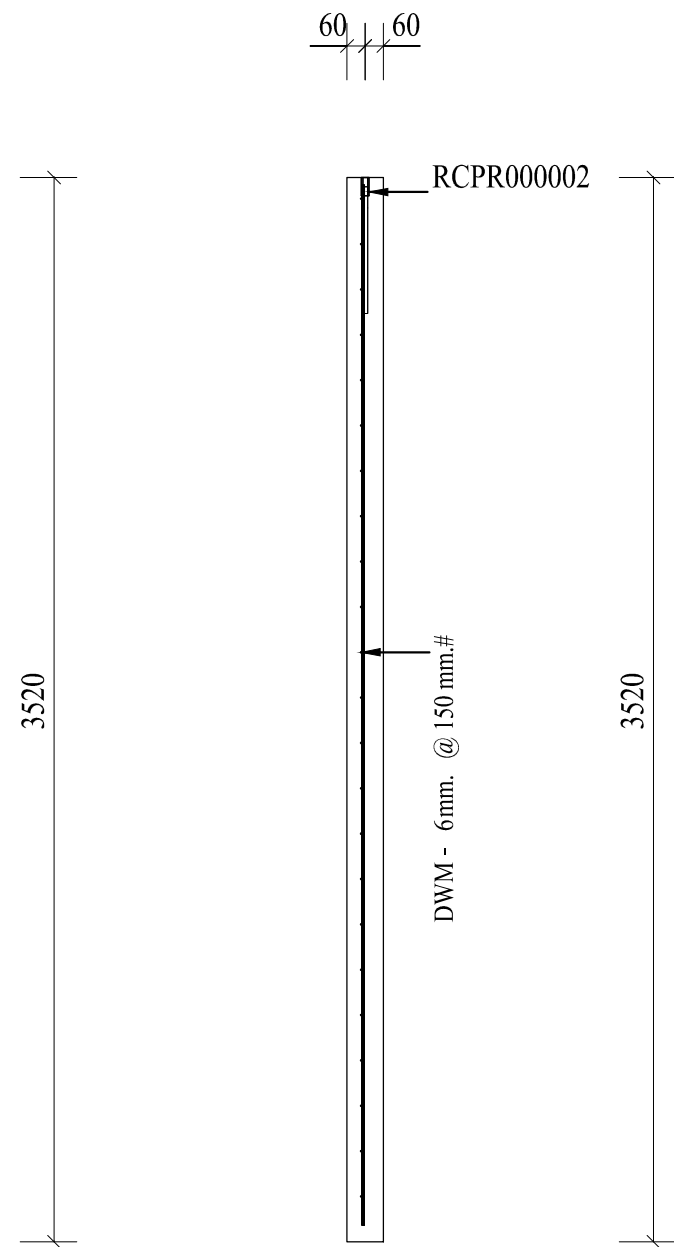
A - A (1:25)
