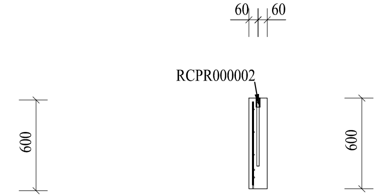
A - A (1:25)
